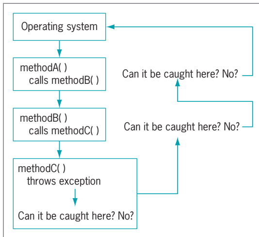
Figure 12-32 Cycling through the call stack
