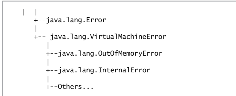
Figure 12-1 The Exception and Error class inheritance hierarchy
